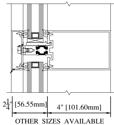
③ Horizontal
