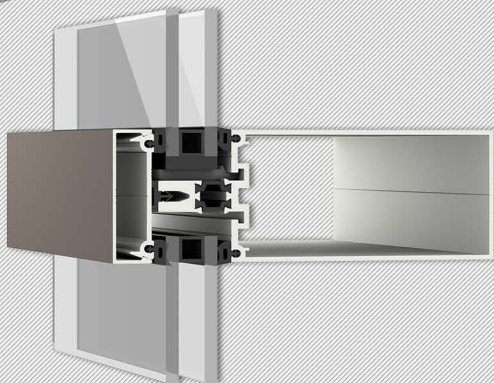
Double Glazed Capped
