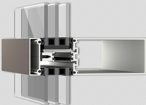
Triple Glazed Capped
