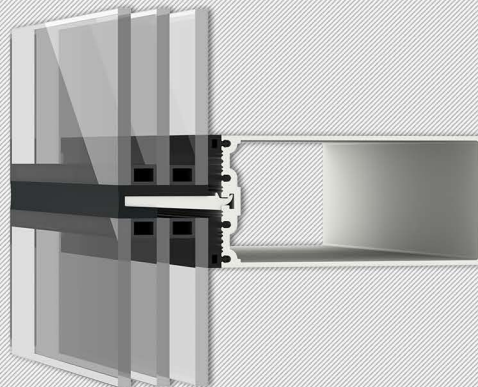
Triple Glazed SSG
