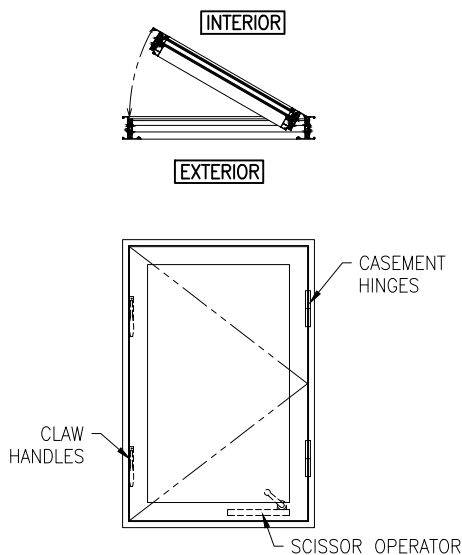
CASEMENT WINDOW OPEN-IN (S.H.O.I.)
