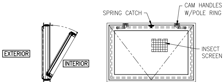
HOPPER WINDOW OPEN-IN (B.H.O.I.)
