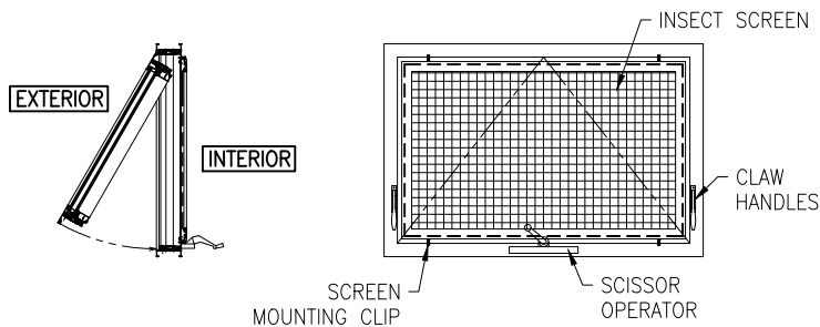
AWNING WINDOW OPEN-OUT (T.H.O.O.)
