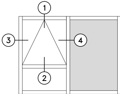
AWNING WINDOW OPEN-OUT (T.H.O.O.)
