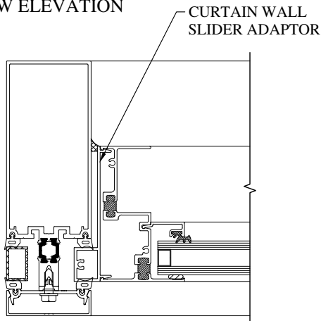
SERIES 740 SEALED UNITS WINDOW ELEVATION
