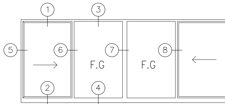
SERIES 720 SEALED UNITS WINDOW ELEVATION
