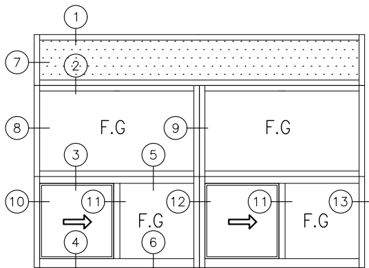
TYPICAL WINDOW ELEVATION
