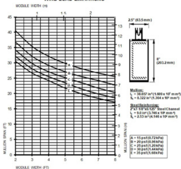
SERIES 5500 (2 1/2" x 8" Back Bar) & 1/8" Formed Steel Channel
