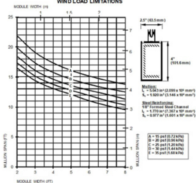
SERIES 5500 (2 1/2" x 4" Back Bar & 1/8" Formed Steel Channel) WIND LOAD LIMITATIONS
