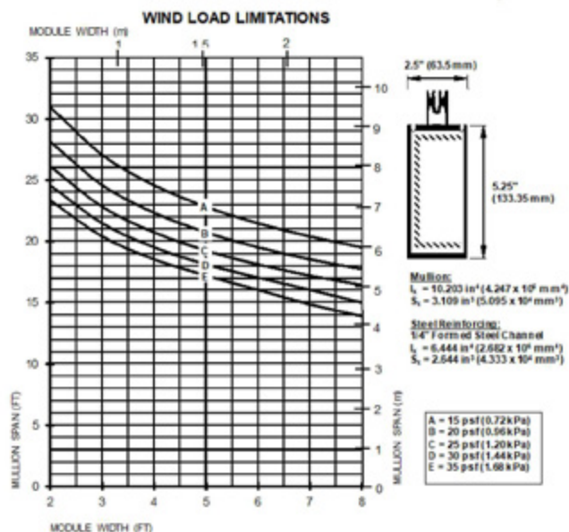
SERIES 5500 (HEAVY DUTY) (2 1/2"x5 1/4" Back Bar & 1/4" Formed Steel Channel)
