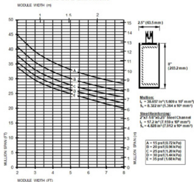
SERIES 5500 (2 1/2" x 8" Back Bar) & 1/4" Formed Steel Channel
