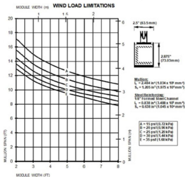
SERIES 5500 (2 1/2" x 2 7/8" Back Bar & 1/8" Formed Steel Channel) WIND LOAD LIMITATIONS
