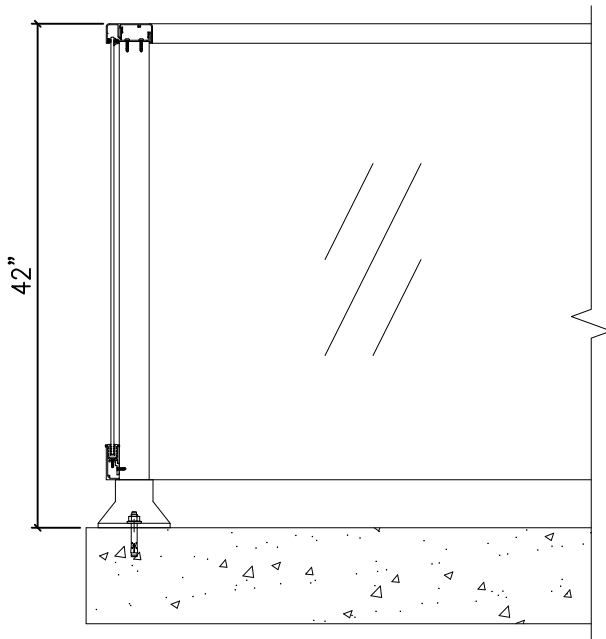
FLOOR MOUNTING
