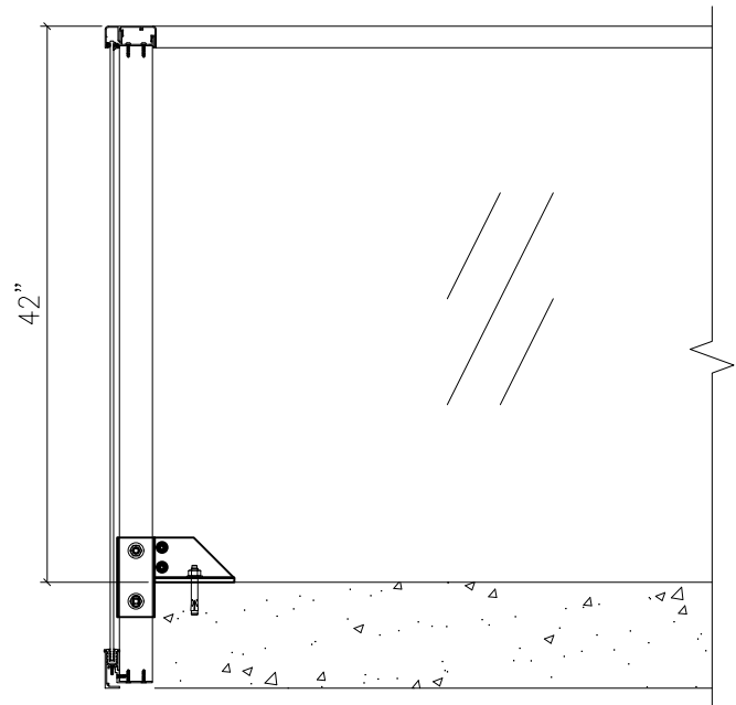
BY-PASS MOUNTING
