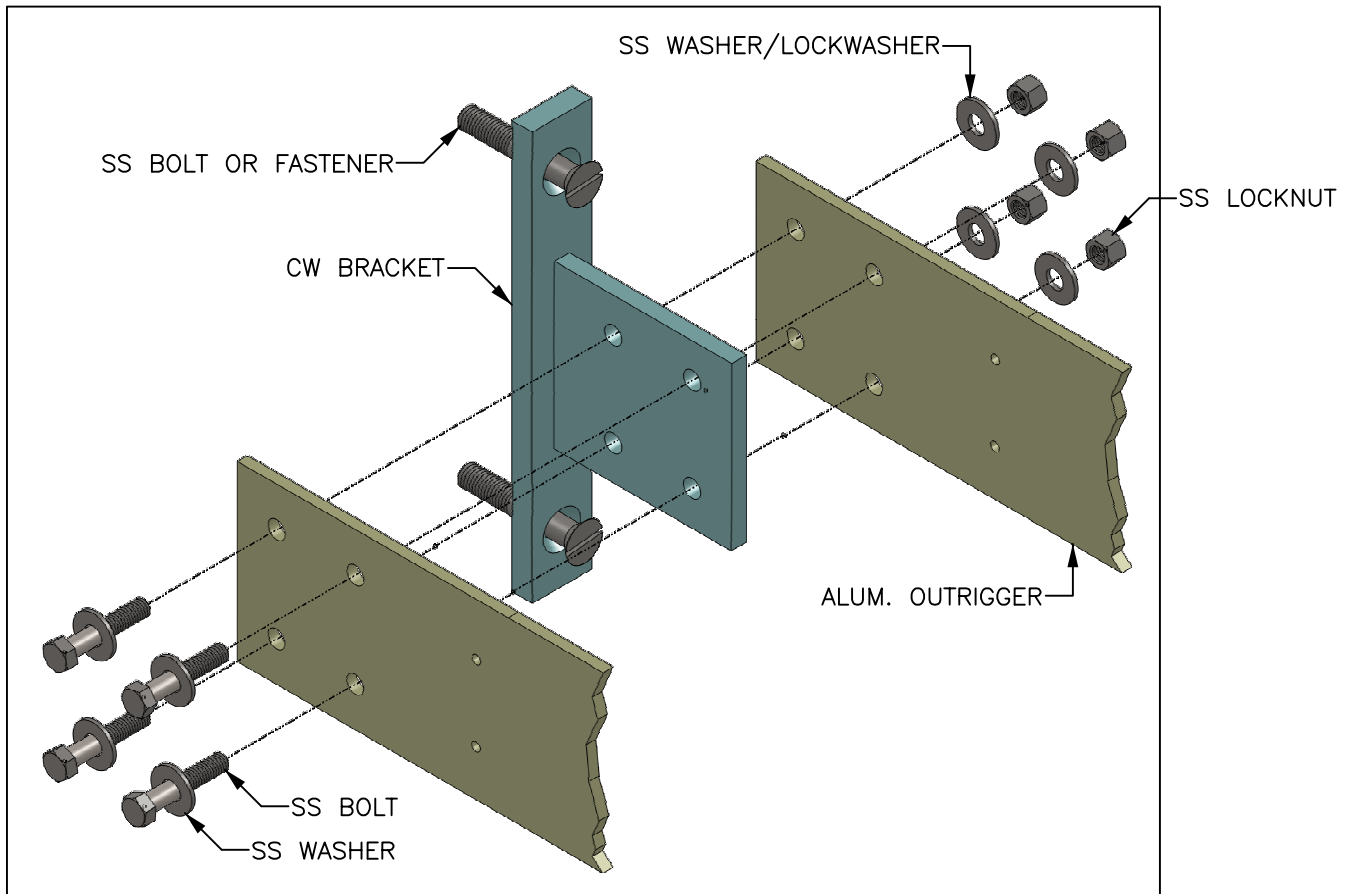
OUTRIGGER TO BRACKET CONNECTION EXPLODED ISOMETRIC VIEW
