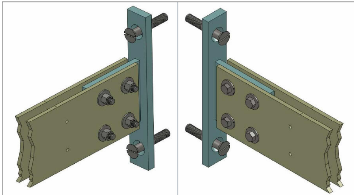
OUTRIGGER TO BRACKET CONNECTION FULLY ASSEMBLED ISOMETRIC VIEW
