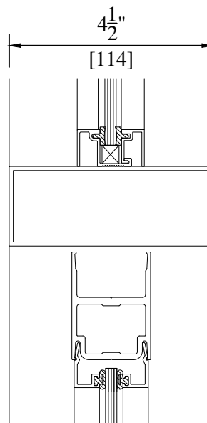
Std. Concealed Closer with Center Hung Door
